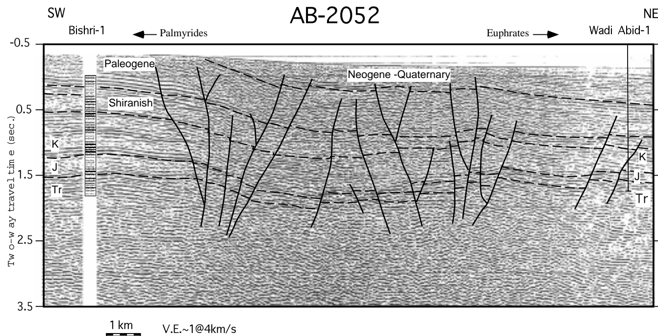
Fig. 11. Portion of seismic line showing complex fault system at northern edge of Bishri block. Interpretation constrained by well data including synthetic seismogram in Bishri-1 well. Note thickening of Mesozoic section from Wadi Abid to Bishri wells. Neogene uplift of Bishri block thus appears to have reactivated bounding fault zone of Mesozoic Palmyride trough. Migrated using a finite difference algorithm. Location shown in Fig. 3.
