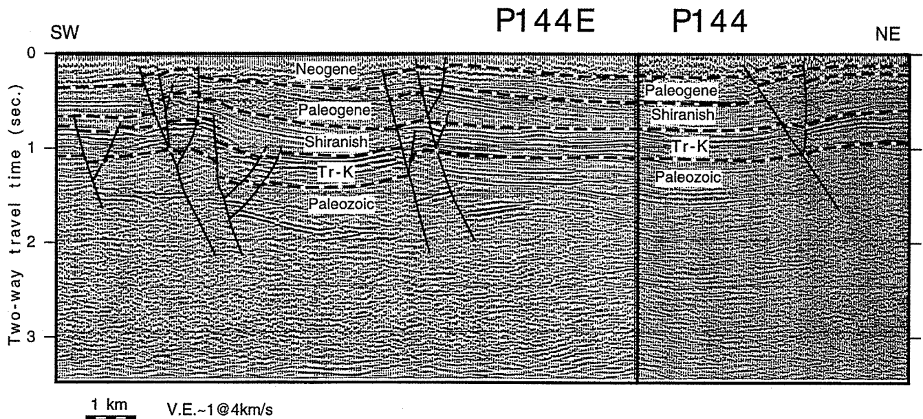
Fig. 13. Portion of seismic line showing thickening of Shiranish formation on upthrown fault blocks, indicating Neogene compressional or transpressional reactivation of Late Cretaceous extensional or transtensional faults. Migrated using a finite difference algorithm. Location shown in Fig. 3.
